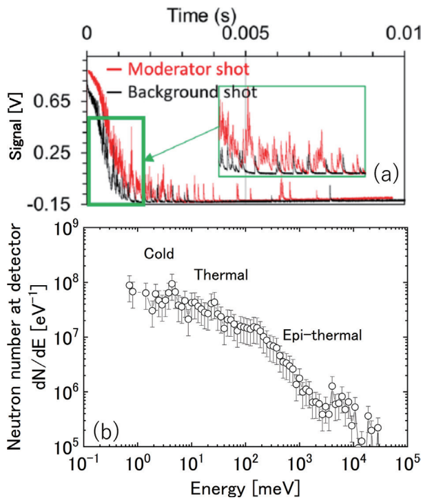
Fig. 3 Time-of-flight signal (a) and the energy spectrum (b) of neutrons from the solid hydrogen moderator. 3) The figure (a) is adopted from Ref. 3).
