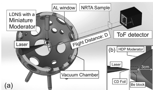
Fig. 8 (a) Setup of the neutron resonance spectroscopy by the LDNS at LFEX laser facility. (b) The miniature moderator.
