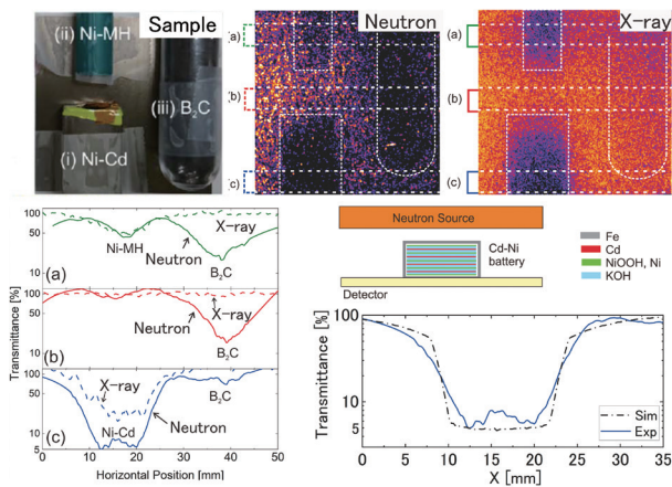
Fig. 5 (Upper) Samples used for the simultaneous radiography with thermal neutrons and x-ray and the experimental results obtained in a single laser shot. (Lower) The transmittance of neutrons and x-rays along the horizontal lines shown as (a) ~ (c) in the radiography pictures. The neutron transmittance for the Ni-Cd battery is compared with the simulation to analyze the thickness of the cadmium. The figures are adopted from Ref. 2).
