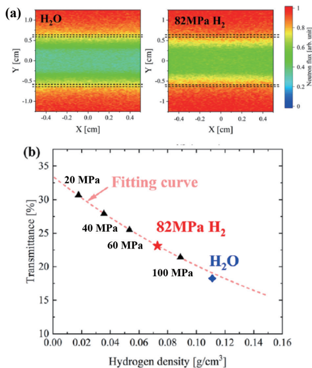
Fig. 7 (a) Simulated transmittance of thermal neutrons for the stainless steel pipes fulfilled with H 2 O at 1 atm. and H 2 gas at 82 MPa. (b) The experimental neutron transmittance for the water compared with the simulated ones for H 2 gas as a function of the hydrogen density. The figures are adopted from Ref. 5).
