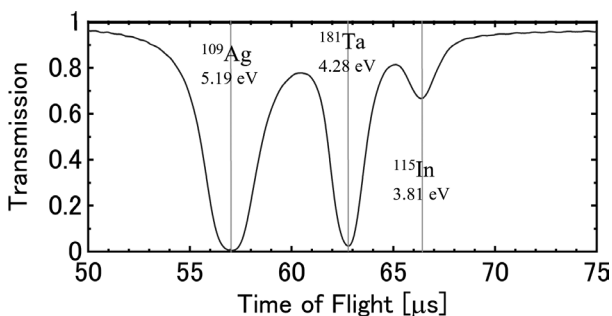
Fig. 9 Theoretical transmittance of neutrons indicating the dips attributed to the neutron resonance absorption.
