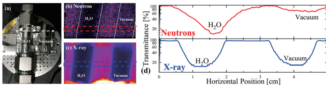
Fig. 6 (a) Picture of the stainless steel pipes, of which one is fulfilled with H 2 O at 1 atm. and the another is opened in vacuum chamber. The images measured with thermal neutrons (b) and x-ray (c) obtained in a single laser shot. (d) Transmittances for neutron (red) and x-ray (blue) along the horizontal area surrounded by the dashed lines in the images. The figures are adopted from Ref. 5).
