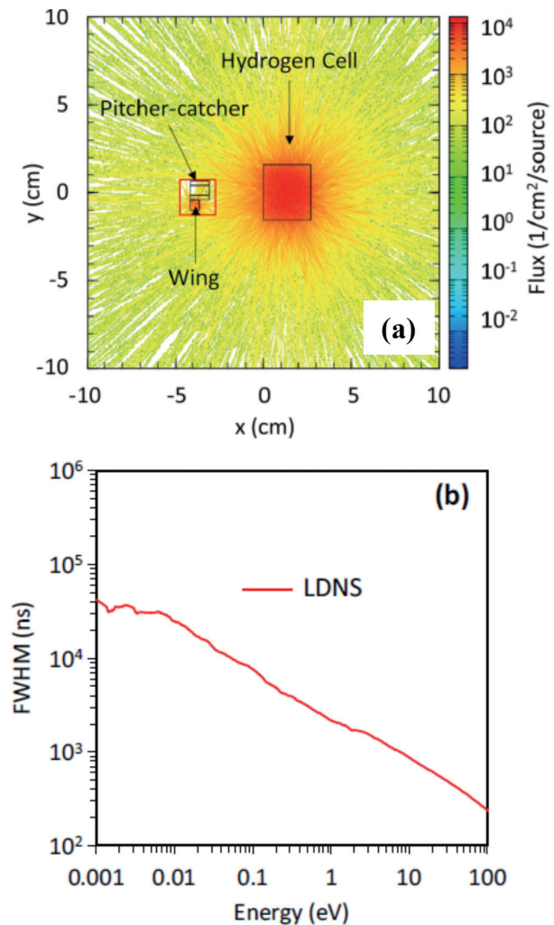
Fig. 4 Spatial distribution of neutrons below 25 meV (a) and the pulse duration of neutrons at the exit of the solid hydrogen moderator (b) simulated by PHITS code. The figures are adopted from Ref. 3).
