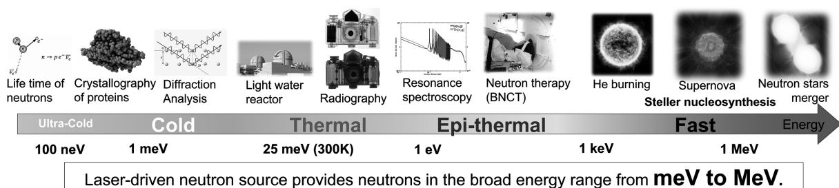
Fig. 2 Energy range of neutrons available in the laser-driven neutron source.
